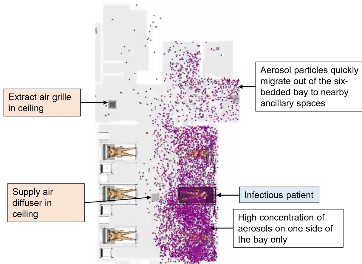
CFD simulation of six-bedded bay in a large teaching hospital showing the migration of 2.5µm aerosol particles exhaled by an infectious patient after 10 minutes. (Source: AAirDS study)
