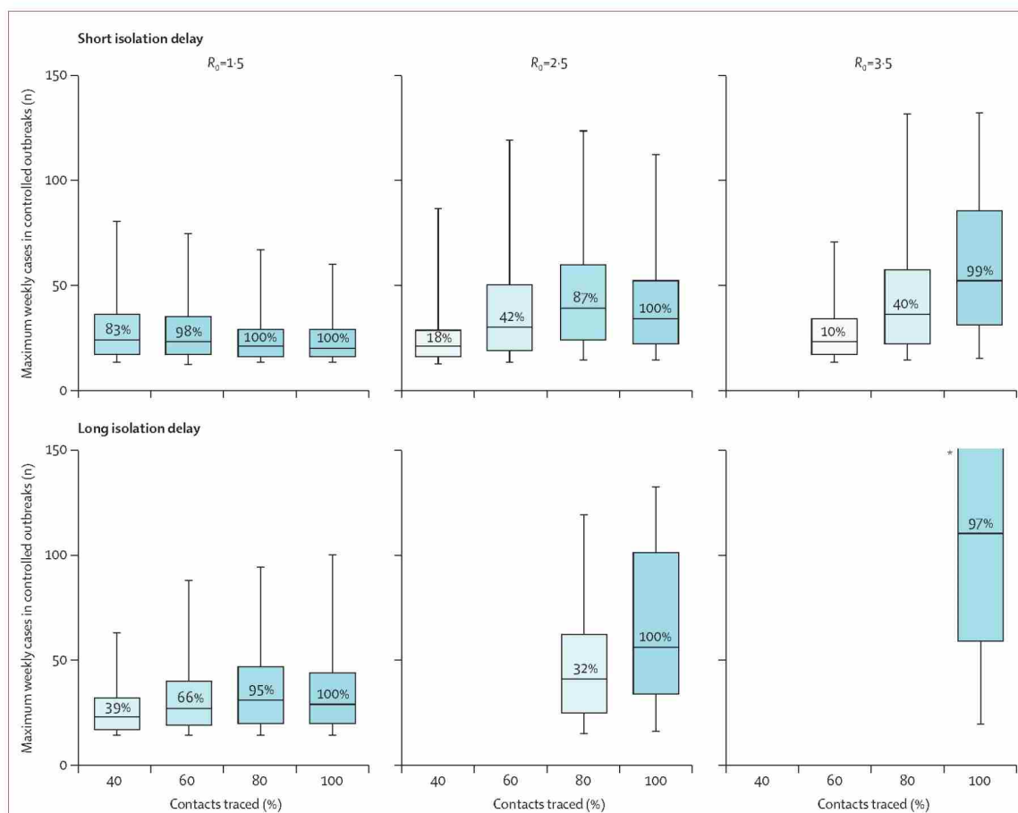
Figure 5: The maximum weekly cases requiring contact tracing and isolation in scenarios with 20 index cases that achieved control within 3 months Scenarios vary by reproduction number and the mean delay from onset to isolation. 15% of transmission occurred before symptom onset, and 0% subclinical infection. The percentage of simulations that achieved control is shown in the boxplot. This illustrates the potential size of the eventually controlled simulated outbreaks, which would need to be managed through contact tracing and isolation. *The interval extends out of the plotting region.
