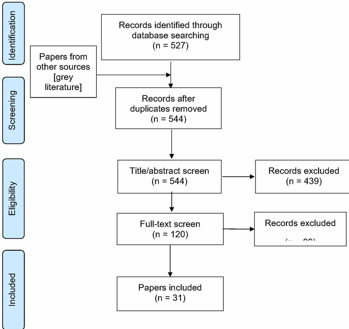
Figure 1. PRISMA diagram
