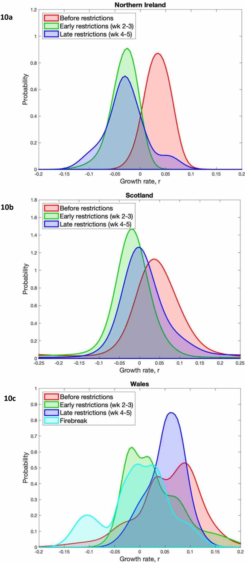
Figures 10a-c: Plots showing, for each nation, the sum of the growth rate probability densities across all LTLAs, before, immediately after, and some time after restrictions.
