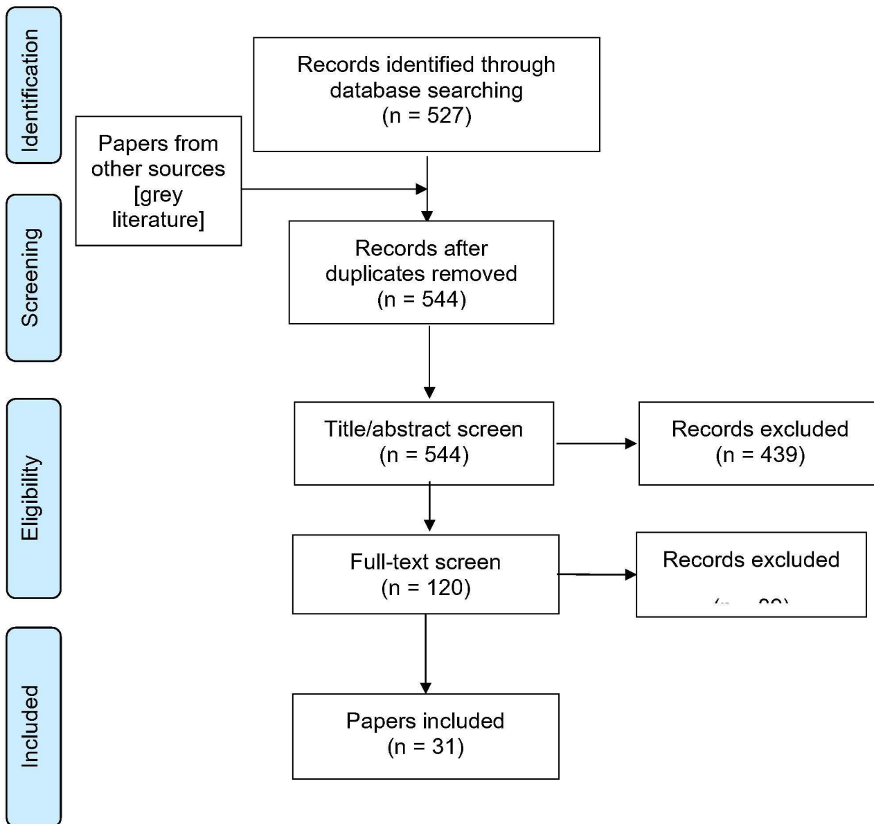
Figure 1. PRISMA diagram
